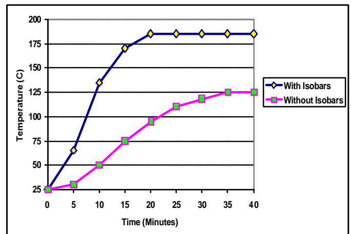
Heating of Core Pins to Steady State Isobar VS. Solid Core Pin
